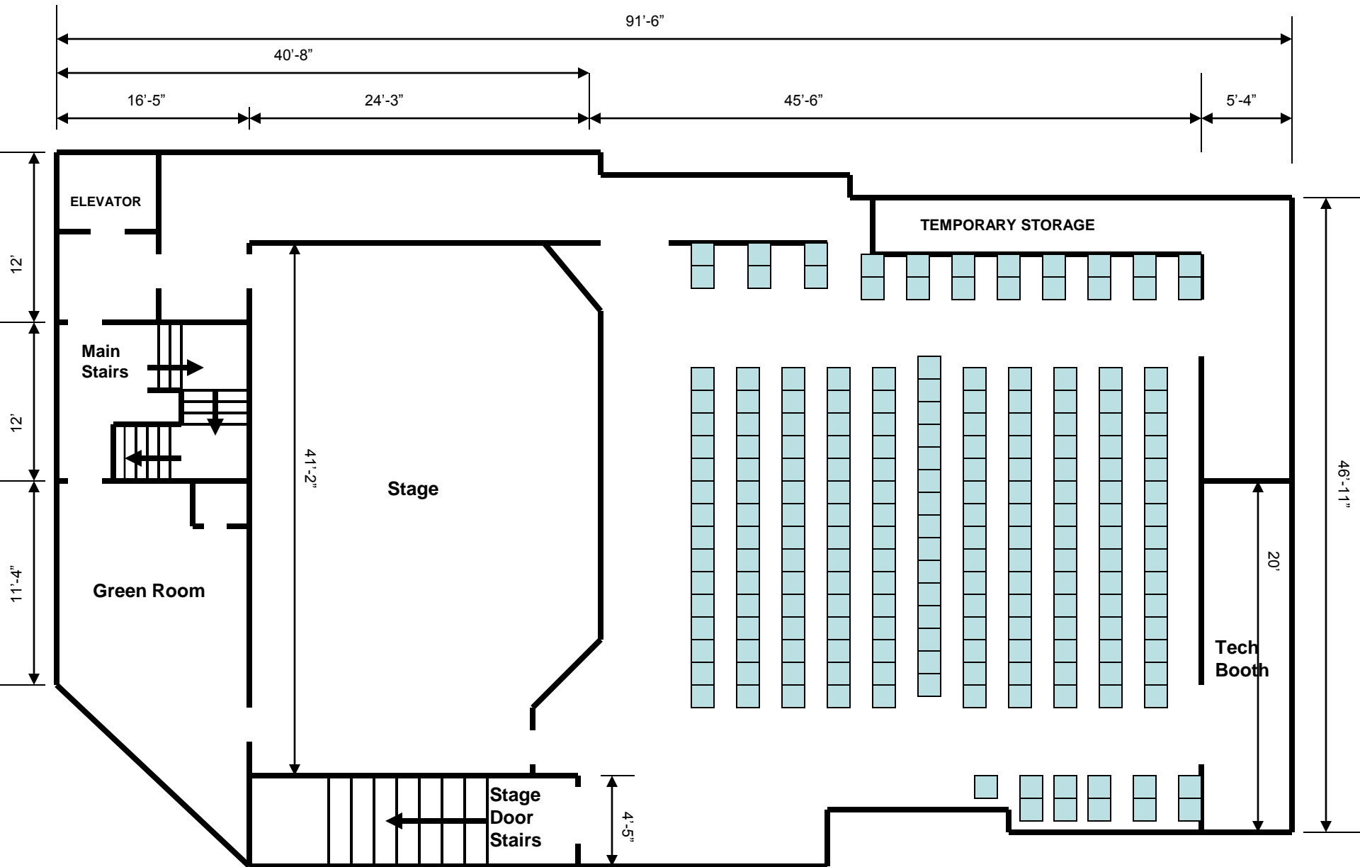
Studio Theatre – Upper Level
